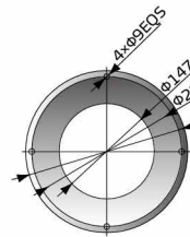
SHR-3U-S Base Flange
